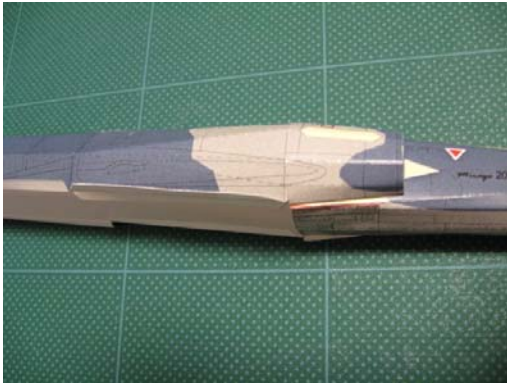
⑲. H:部品の折り方。 Folding line of H parts.
